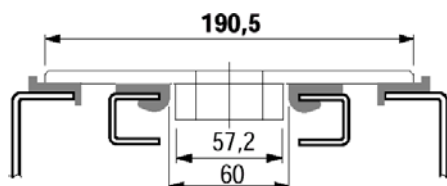
Guiding of stainless Heavy Duty chains
