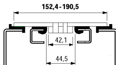
Guiding of 6"-7.5" plastic chains
