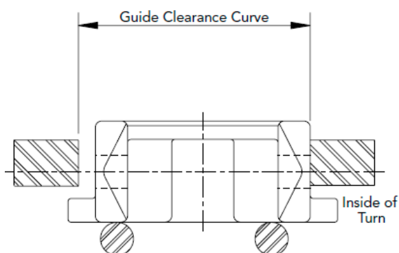
Typical construction – Corner section utilizing corner track
